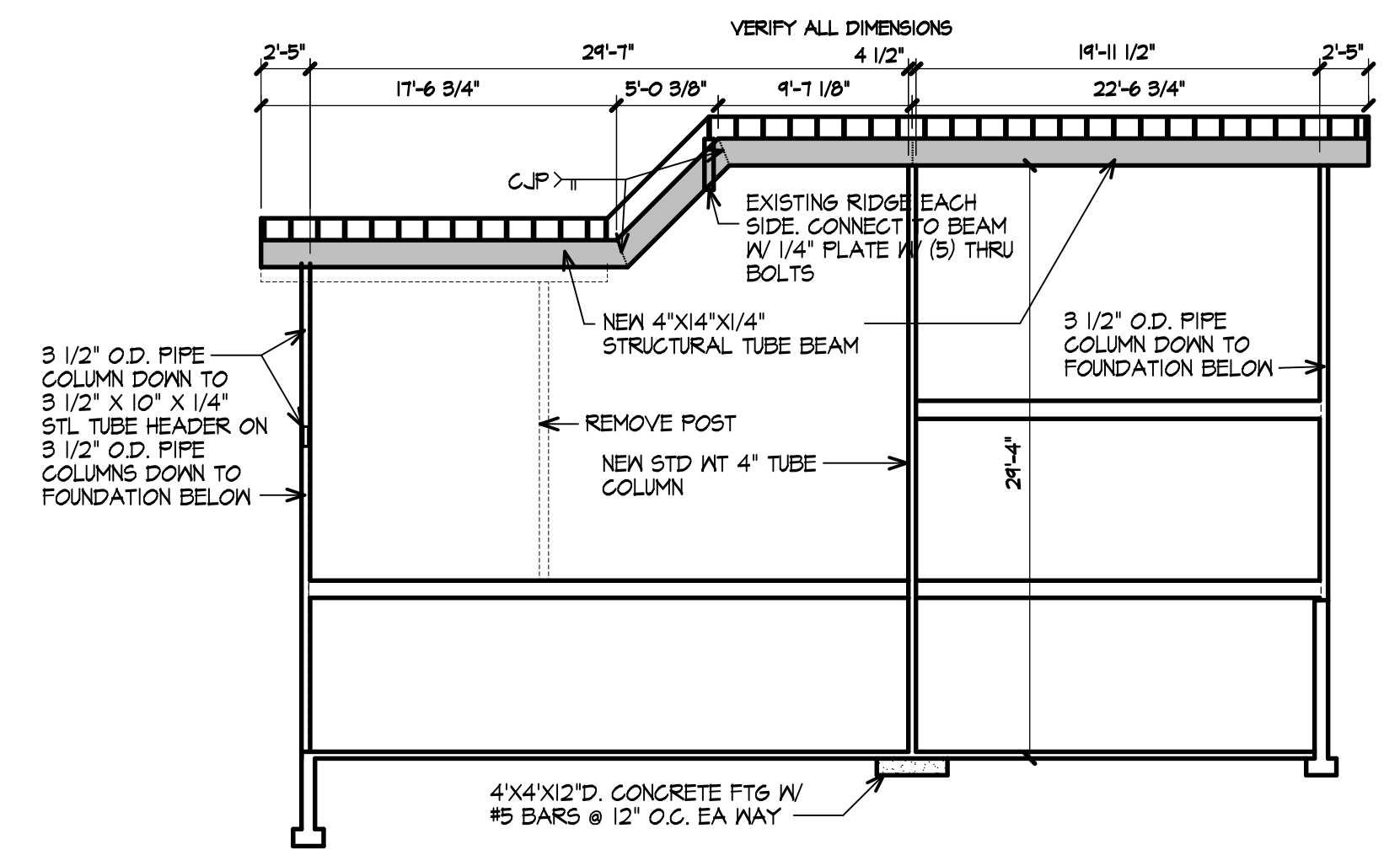
3 A5 Building Section 1/8"=1'-0" 0 2' 4' 8' 12' 16'
