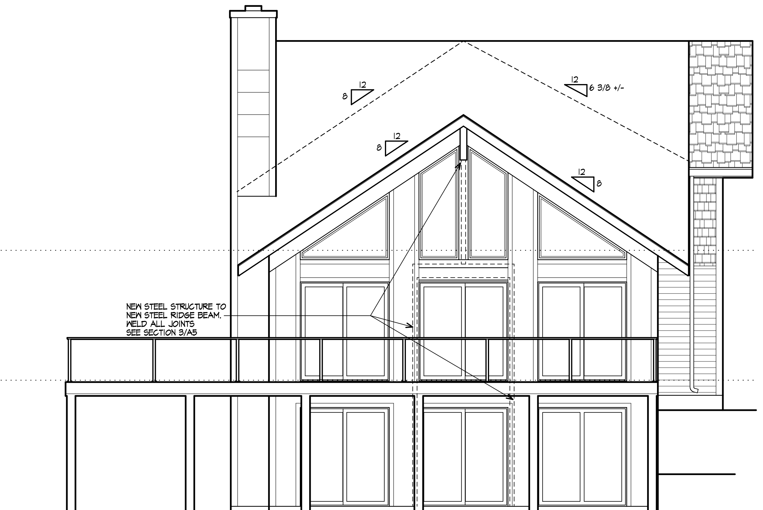
South Elevation
