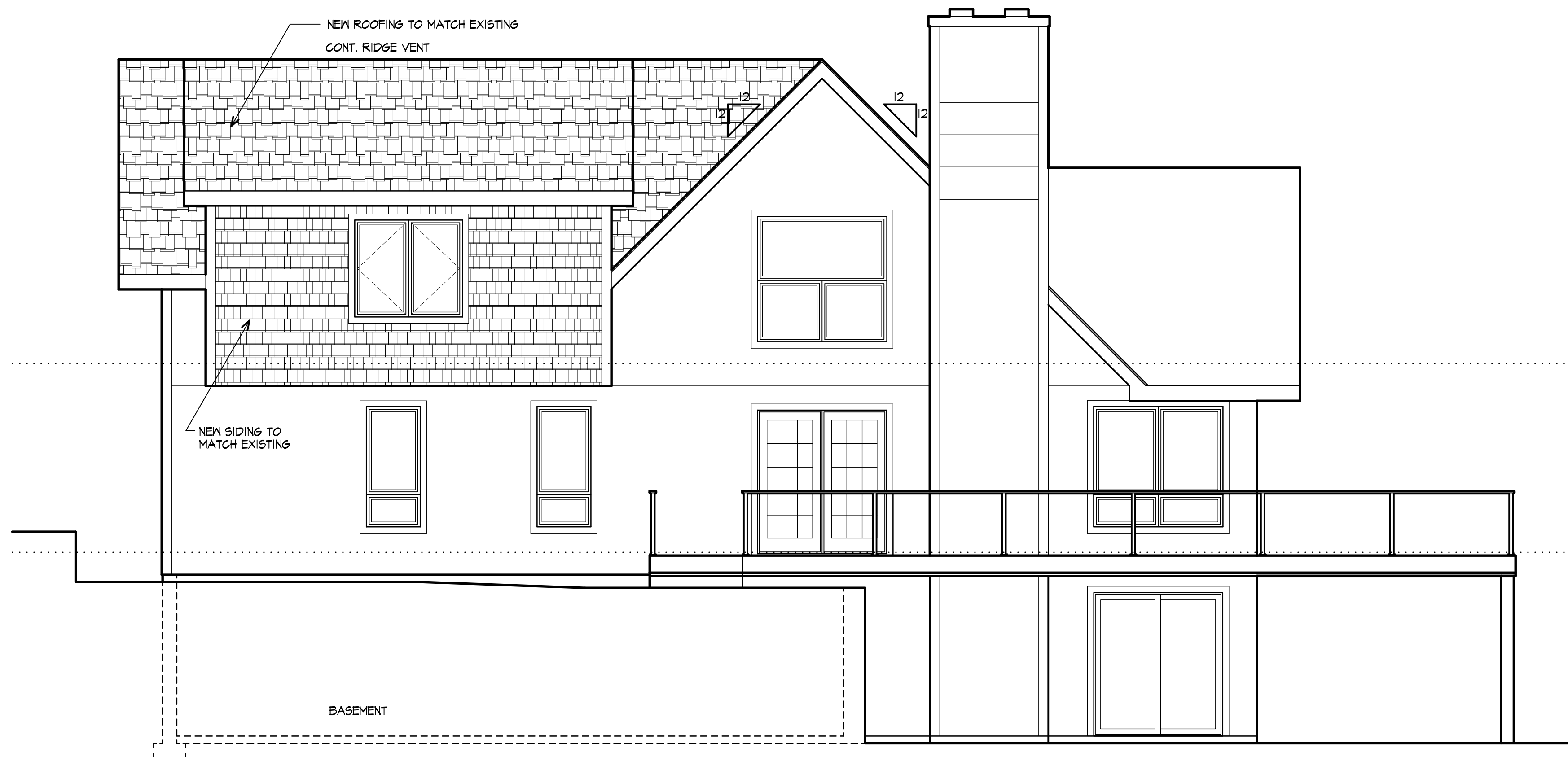
Front Elevation
