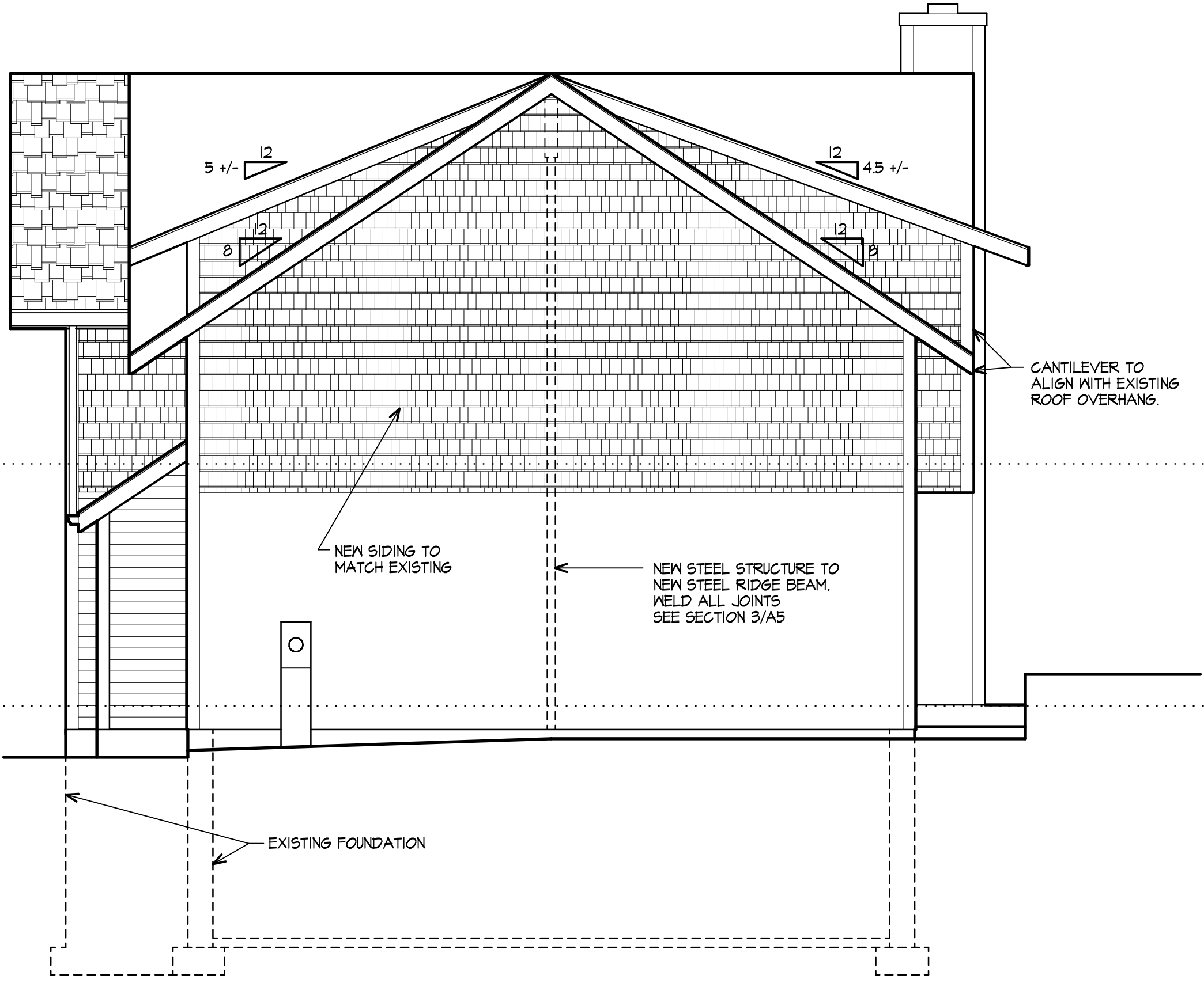
North Elevation
