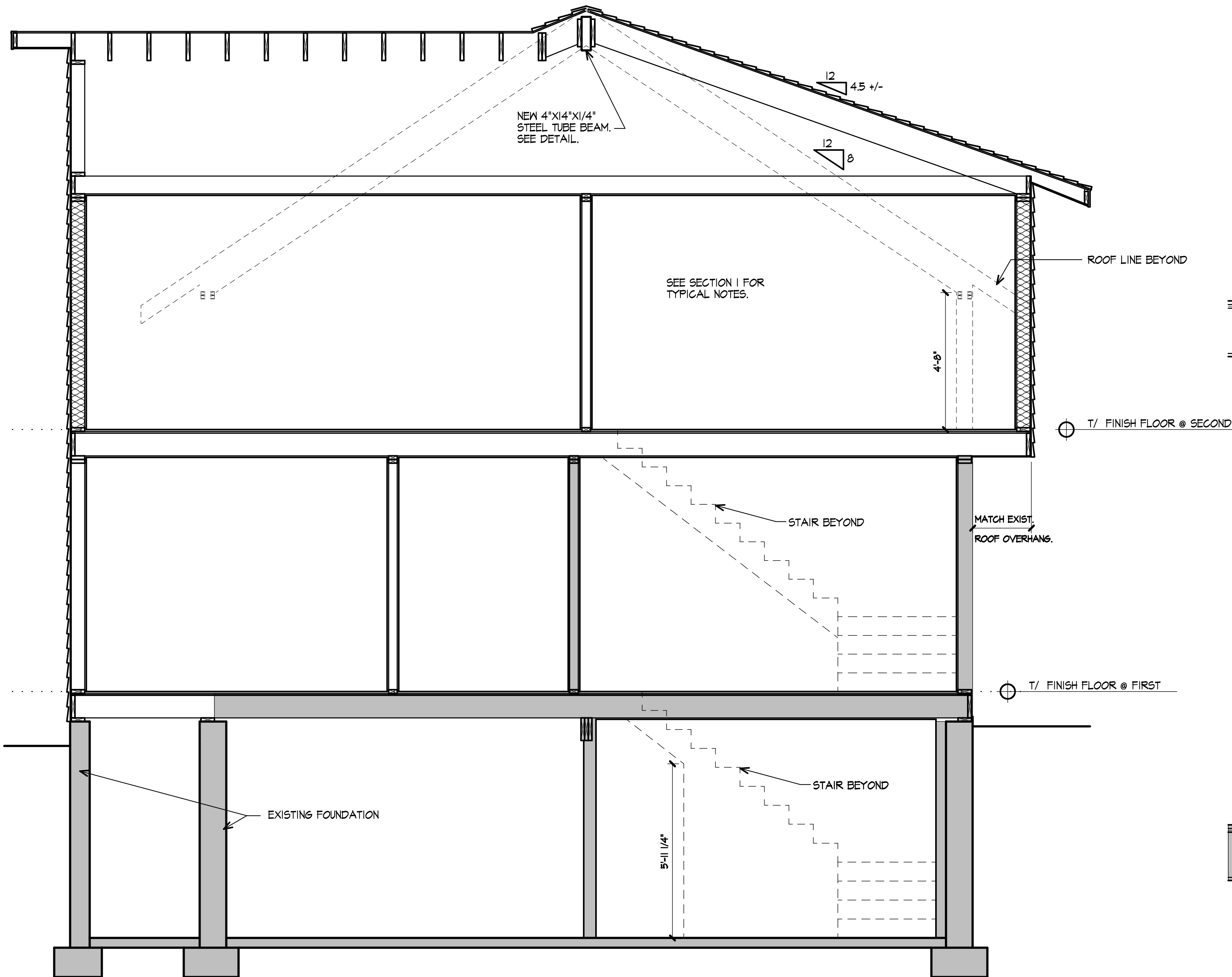
2 A5 Section 3/8"=1'-0" 0 6" 1' 2' 3' 4'
